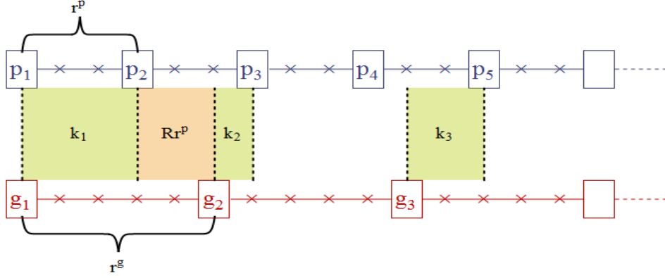
FIGURE 4. The rigid stage game - an example of timing of moves with r^g = 5 and r^p = 3 , illustrating the variables k_n, n^i , and R .
