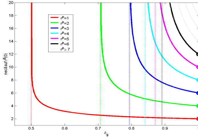
FIGURE 5. Dependence of \overline{r^g}(0) on r^p and \delta_g (from (13) and (14) for the specific game (6)). The dotted asymptotes show the \overline{\delta_g}(0) thresholds.
