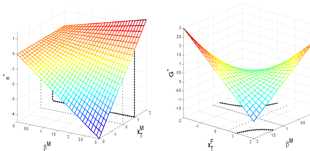
FIGURE 2. Equilibrium policy setting: inflation \pi^* (the left panel) and deficit G^* (the right panel) as functions of the output target values ( x_T^M and x_T^F respectively) and M policy conservatism \beta^M ; under x_T^F = \beta^F = \mu = 1, \rho = 0.5 in the left panel, and x_T^M = 0.5, \beta^F = 1, \mu = 2, \rho = 1 in the right panel.
