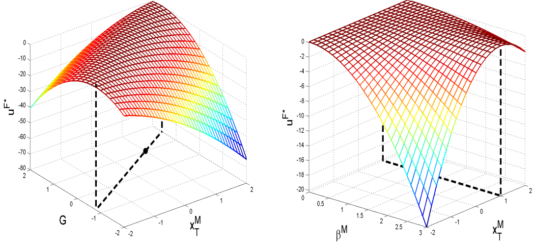
FIGURE 3. Equilibrium F utility and social welfare (assuming u^S = u^F ) as a function of M policy ambition x_T^M , and the deficit G or M policy conservatism \beta^M ; under x_T^S = x_T^F = \beta^M = \rho = 1, \mu = 1.5 in the left panel, and x_T^S = x_T^F = \beta^F = \mu = 1, \rho = 0.5 in the right panel.
