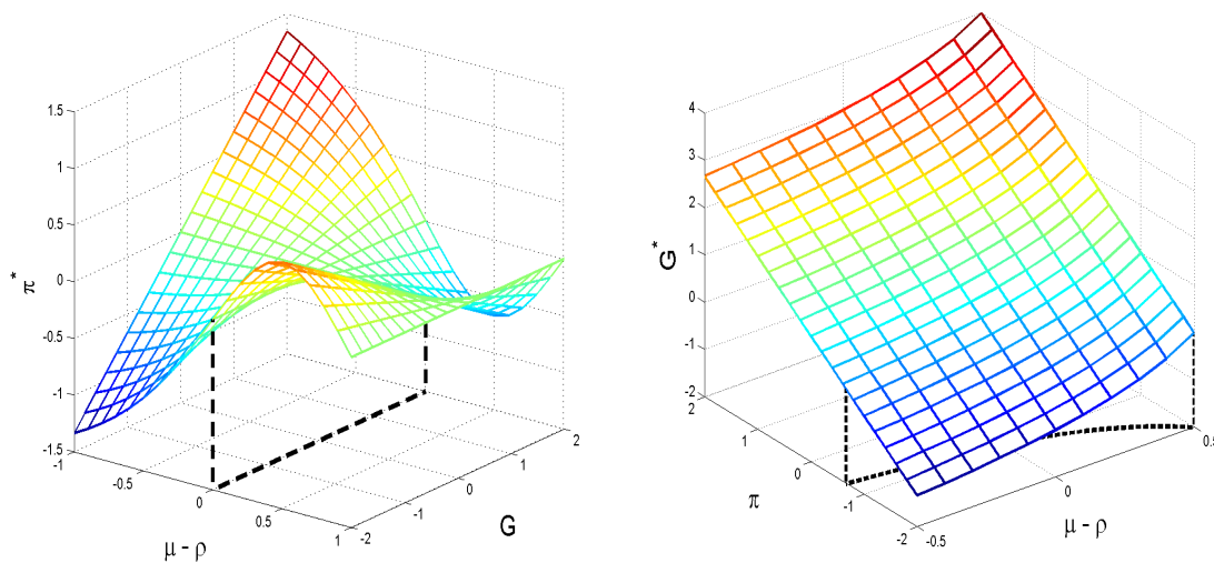
FIGURE 1. M and F policy reaction functions: Optimal inflation \pi^* (the left panel) and deficit G^* (the right panel) as functions of the setting of the other policy and their relative potency \mu - \rho ; under x_T^M = 0, x_T^F = \beta^M = \beta^F = \mu = 1 .
